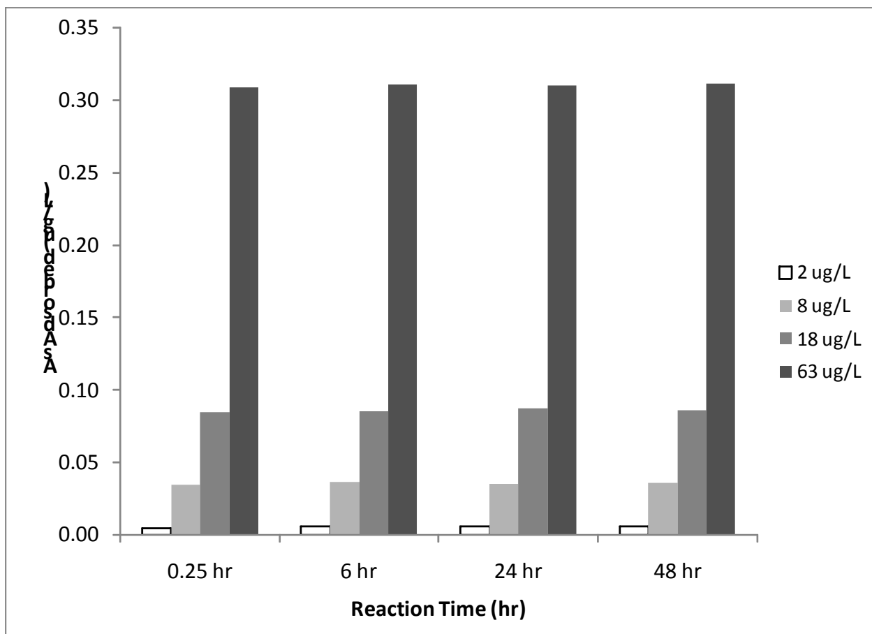
Figure 4. Sediment arsenic adsorption vs. initial standard solution concentrations; pH 8 (study 1). Adsorption results between all standards were significantly statistically different.
