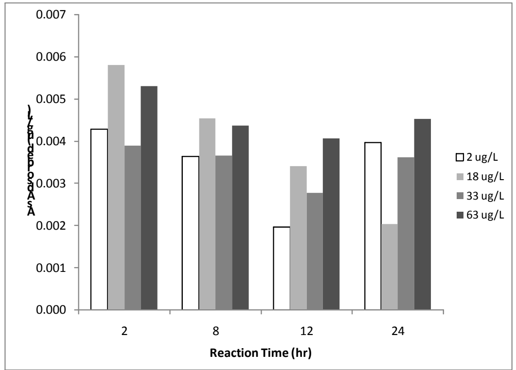
Figure 6. Sediment arsenic adsorption vs. initial standard solution concentrations; pH 5 (study 2). Adsorption results between all standards were significantly statistically different.
