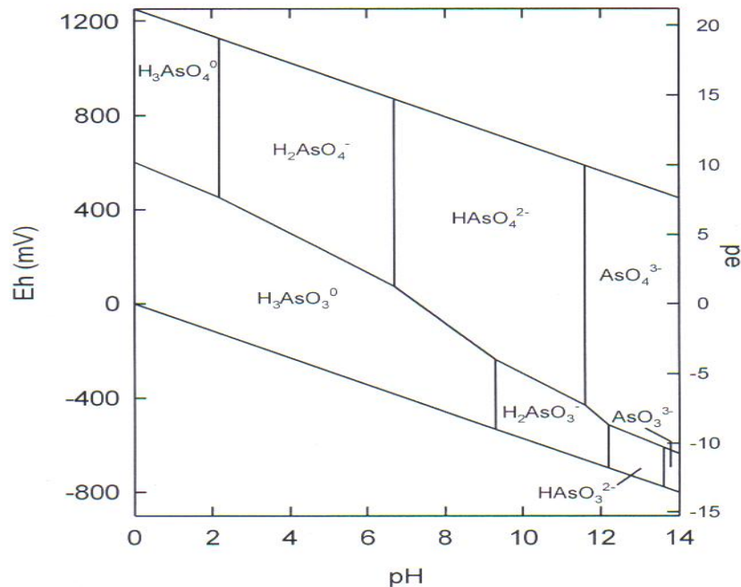
Figure 1. Arsenic Speciation Diagram with Respect to Eh-pH Values (Ringwood, 1996).
