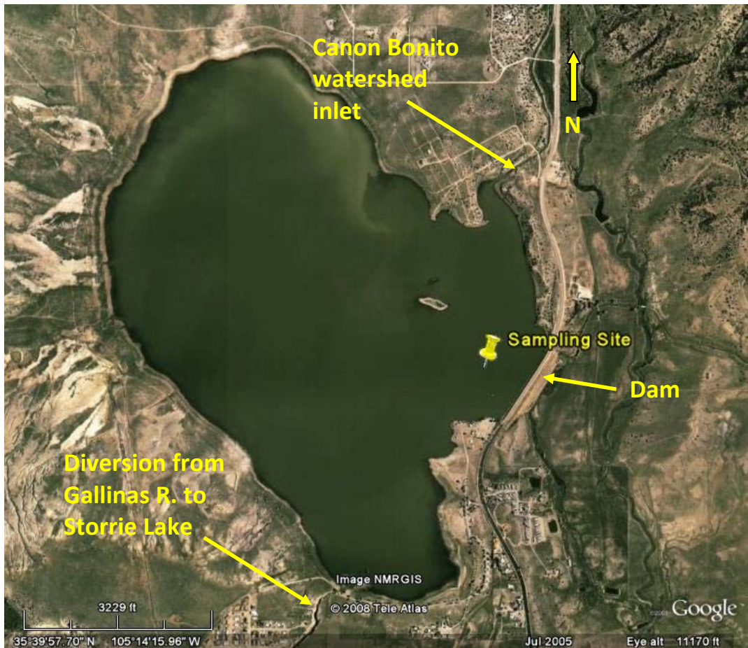
Figure 3. Storrie Lake and sampling location.
