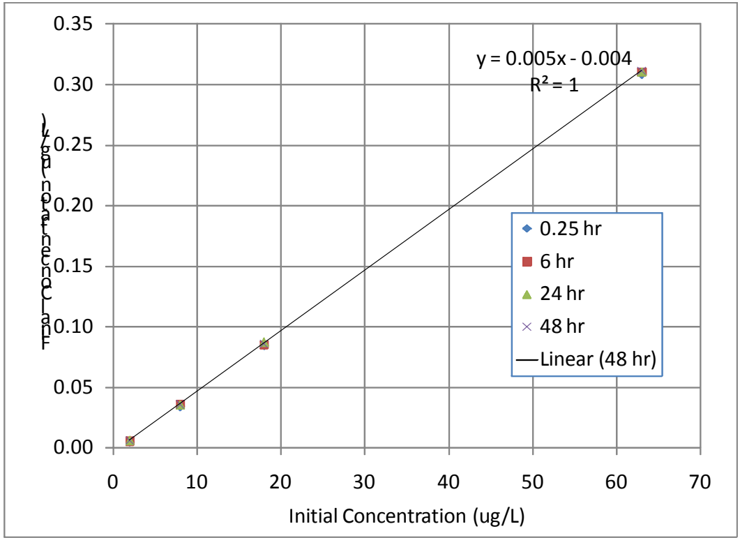
Figure 5. Final solution concentration vs. initial solution concentration; pH 8 (study 1).
