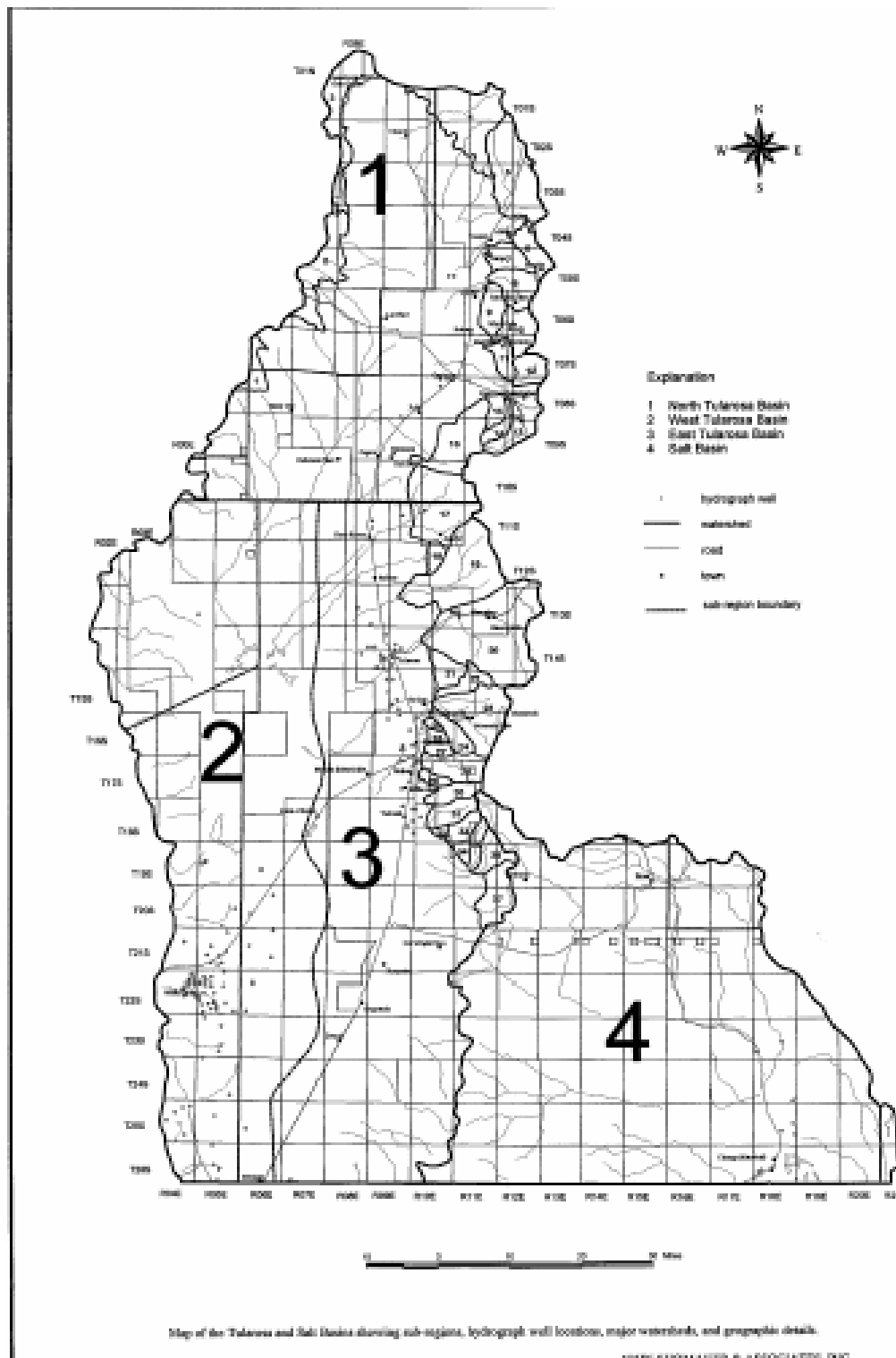
Figure D-2: Sub-basins within the Tularosa Basin (Livingston, 2002)
